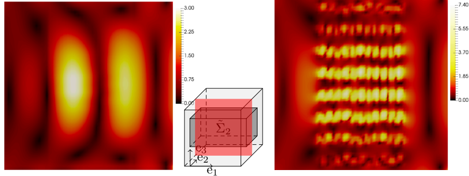
FIGURE 5.3. Metal cuboid \tilde{\Sigma}_2 . We study an e_3 -polarized incident H -field and plot the magnitude of \text{Re}(\hat{H}) (left) and \text{Re}(H^\eta) (right) in the plane x_2 = 0.545 . The analysis (PC) predicts transmission in this case, the analysis (HC) does not exclude transmission. Middle: Microstructure in the unit cube with visualization plane in red.
