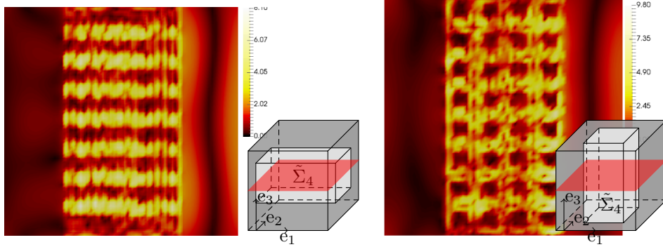
FIGURE 5.5. Metal block with holes. Left: The structure \tilde{\Sigma}_4 , we plot the magnitude of \text{Re}(H^\eta) in the plane x_3 = 0.545 for e_3 -polarized incoming H -field. The analysis (PC) predicts no transmission, the analysis (HC) cannot exclude transmission. Right: A geometry in which the cylinders \tilde{\Sigma}_4 are rotated in e_3 -direction. We plot the magnitude of \text{Re}(H^\eta) in the plane x_3 = 0.5 for e_3 -polarized incoming H -field. Small pictures show the microstructures in the unit cube and the visualization planes in red.
