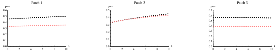
FIGURE 6. Equilibrium T. cruzi prevalence vs. vector migration rate multiplier for infected vectors moving south only; dark curve represents vectors, light curve represents hosts
