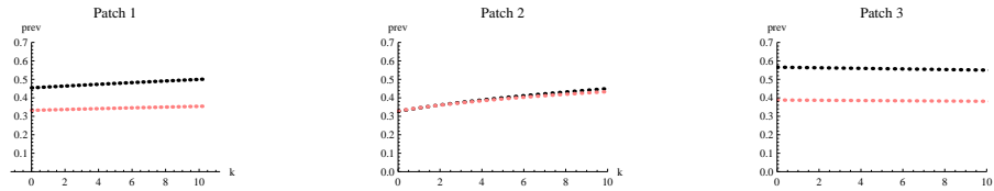
FIGURE 8. Equilibrium T. cruzi prevalence vs. vector migration rate multiplier for all vectors moving south only; dark curve represents vectors, light curve represents hosts
