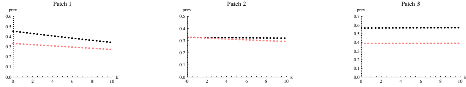
FIGURE 3. Equilibrium T. cruzi prevalence vs. vector migration rate multiplier for infected vectors migrating north only; dark curve represents vectors, light curve represents hosts
