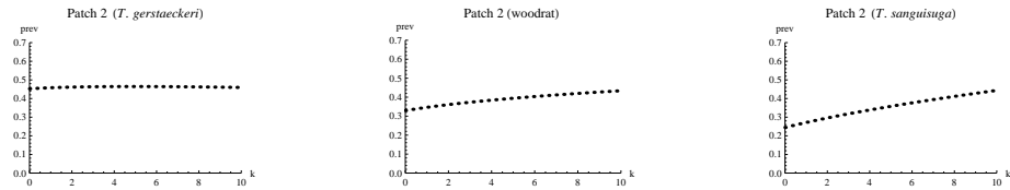
FIGURE 7. Equilibrium T. cruzi prevalence vs. vector migration rate multiplier for infected vectors moving south only (patch 2)
