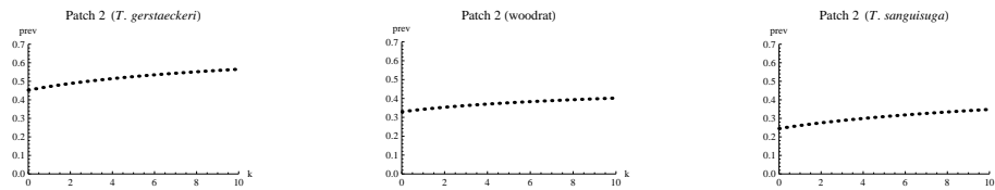
FIGURE 10. Equilibrium T. cruzi prevalence vs. vector migration rate multiplier for infected vectors bidirectional migration (patch 2)
