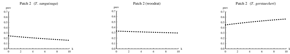
FIGURE 4. Equilibrium T. cruzi prevalence vs. vector migration rate multiplier for infected vectors moving north only (patch 2)
