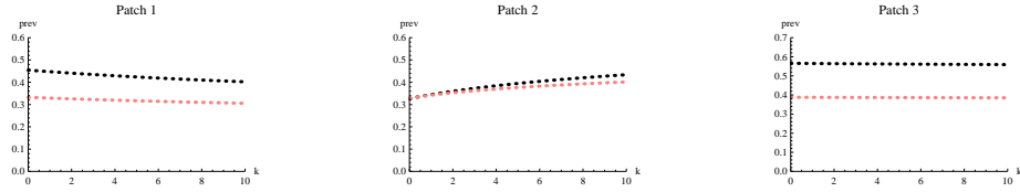
FIGURE 11. Equilibrium T. cruzi prevalence vs. vector migration rate multiplier for all vectors bidirectional migration; dark curve represents hosts, light curve represents vectors
