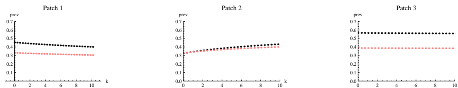
FIGURE 9. Equilibrium T. cruzi prevalence vs. vector migration rate multiplier for infected vectors bidirectional migration; dark curve represents vectors, light curve represents hosts
