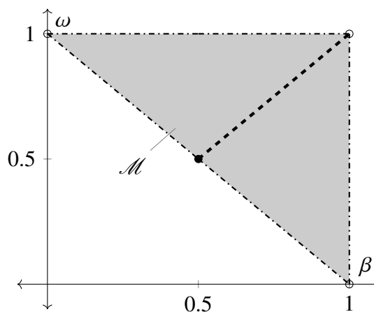
Figure 1. Plot illustration for the set \mathcal{M} .
