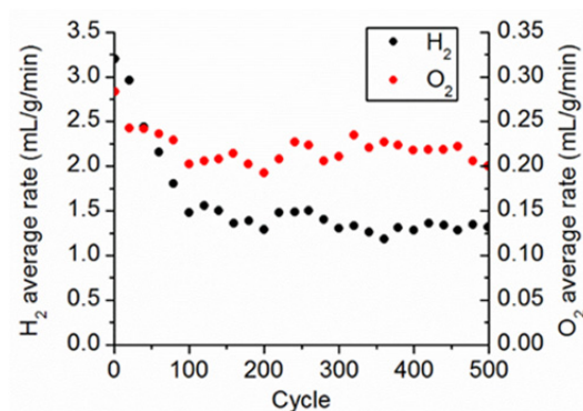
Figure 3. Average O_2 and H_2 production rates over 500 successive cycles performed with ceria, reduction temperature of 1500\text{ }^\circ\text{C} and oxidation temperature of 800\text{ }^\circ\text{C} [40].
