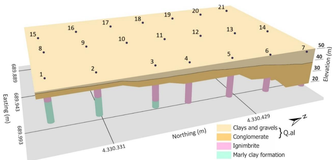
Figure 8. 3D representation of the lithological boundaries determined by the geophysical interpretation.
