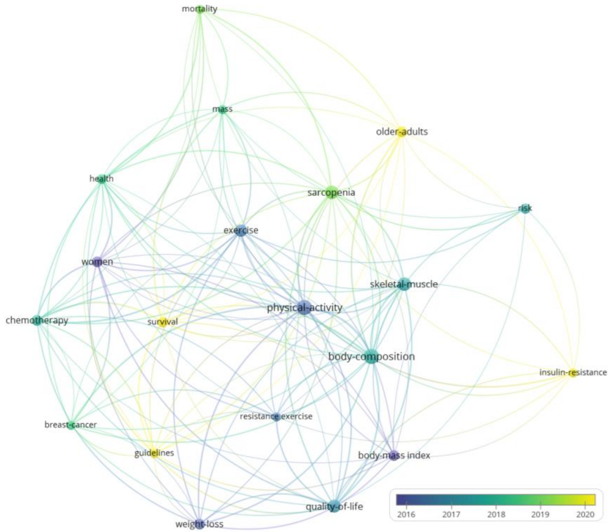
Figure S6. KP AS 5_0 Avg Pub Years.
