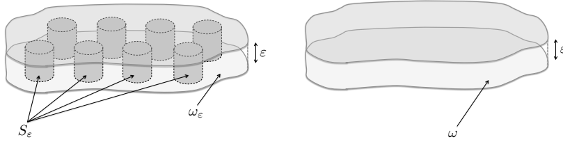
FIGURE 3. Views of the domain \Omega_\varepsilon (left) and \Lambda_\varepsilon (right)
