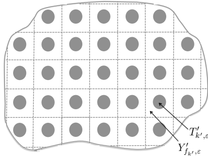
FIGURE 2. View of \omega_\varepsilon
