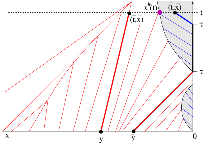
FIGURE 7. The trajectories leading to the maximum value in (3.18). For each time t \geq 0 there exists a unique point x^\sharp(t) \leq 0 with the following property. For terminal points \bar{x} < x^\sharp(t) , optimal trajectories are affine, while for terminal points x > x^\sharp(t) optimal trajectories are piecewise affine, also taking the value x = 0 on some time interval.
