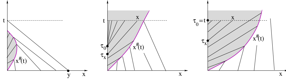
FIGURE 9. Various cases considered in the proof of Proposition 3. Here t \mapsto x^\#(t) is the Lipschitz curve separating characteristics which originate from the x -axis and from the t -axis.
