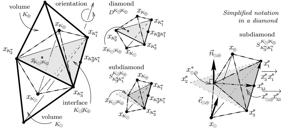
FIGURE 2. Primal volumes, diamond; subdiamond and zoom on it (Version (B) of 3D DDFV mesh)
