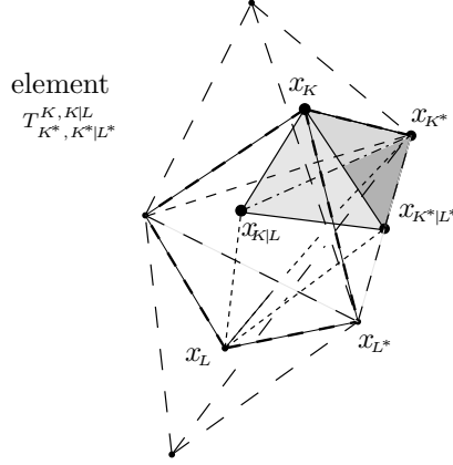
FIGURE 1. One of the twelve elements in diamond D^{K|L} with triangular base K|L
