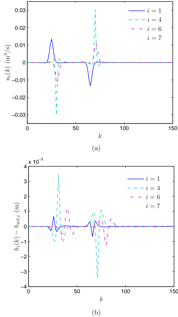
FIGURE 6. Evolution for four representative canal reaches of (a) set-points and (b) deviation of the water levels from reference values.
