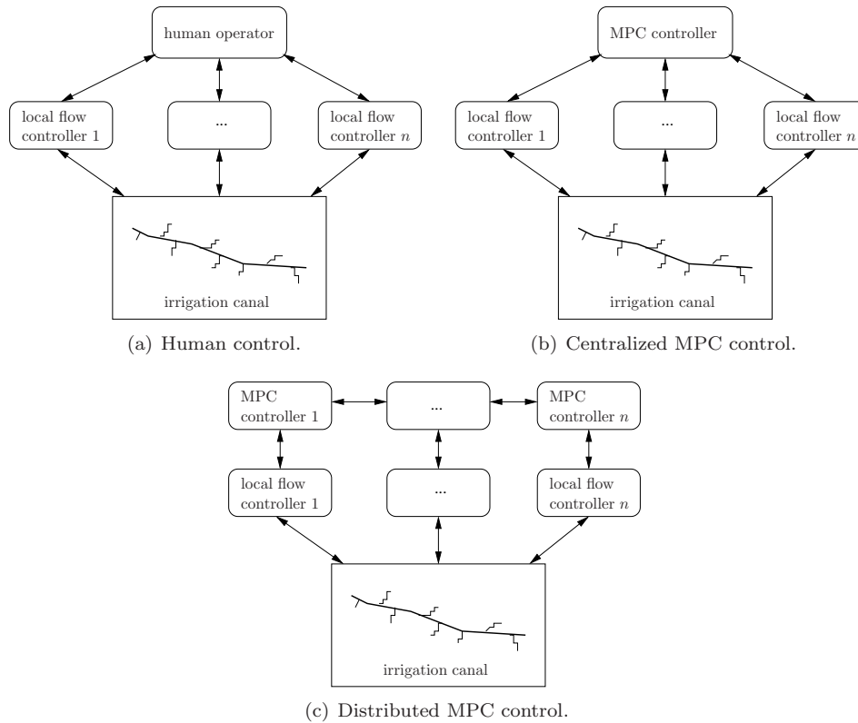
FIGURE 4. Three control configurations for the control of irrigation canals.
