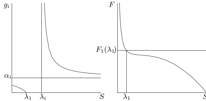
FIGURE 1. Graphical depictions of the hypotheses 2 and 3 in Theorem 2. On the left, hypothesis 2. On the right, hypothesis 3.
