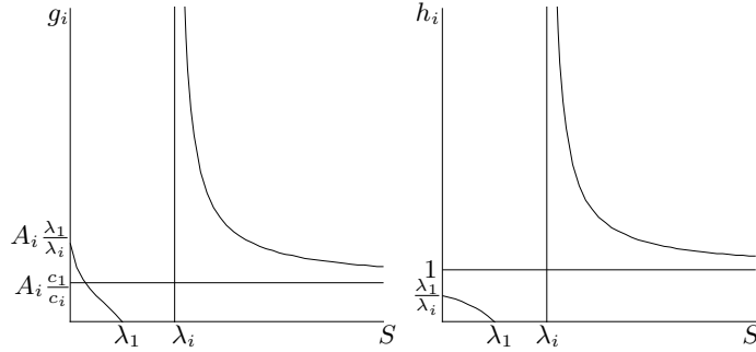
FIGURE 2. On the left, the graph of the function g_i(S) for p_i(S) = \frac{a_i S}{b_i + S} and y_i(S) = Y_i(1 + c_i S) : hypothesis 2 in Corollary 5 is not satisfied. On the right the graph of the function h_i(S) = \frac{S - \lambda_1}{S - \lambda_i} .
