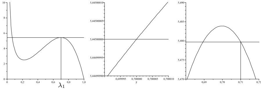
FIGURE 6. On the left, the plot of F_1(S) for (16) or (17) where c = 50 and m_2 = 10 . On the center, the magnification of the neighborhood of \lambda_1 = 0.7 shows that F'_1(\lambda_1) > 0 . On the right, the magnification of the neighborhood of \lambda_1 = 0.71 shows that F'_1(\lambda_1) < 0 .
