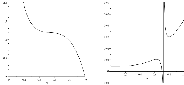
FIGURE 5. Graphical verification of hypotheses 2 and 3 in Theorem 2 for (16) with c = 8 and m_2 = 10 . On the left, the graph of the function F_1(S) . On the right the graph of the function g_2(S) .
