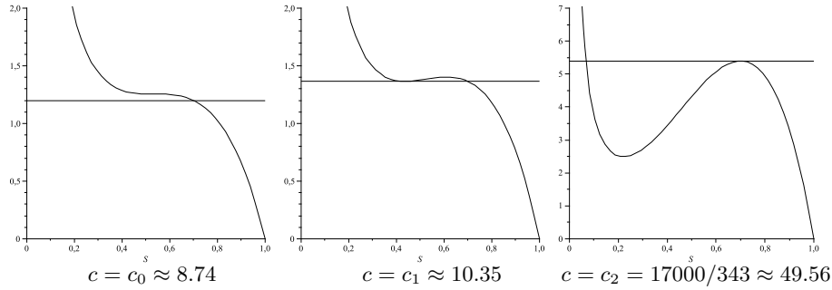
FIGURE 4. Graphs of the function F_1(S) for p_1(S) = 2S/(0.7 + S) and y_1(S) = 1 + cS^3 in the cases c = c_0, c_1, c_2 .
