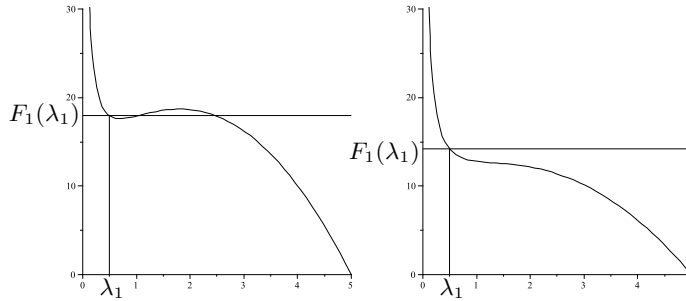
FIGURE 3. The graph of the function F_1(S) for p_1(S) = \frac{a_1 S}{b_1 + S} (where a_1 = 2.1/1.1 , b_1 = 0.5/1.1 and \lambda_1 = 0.5 ) and y_1(S) = Y_1(1 + c_1 S) . On the left, the case c_1 = 1.8 for which hypothesis \beta in Corollary 5 is not satisfied. On the right, the case c_1 = 1 for which this hypothesis is satisfied.
