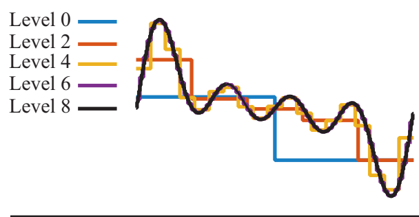
Figure 2. Simple surface representation using Haar wavelets.
