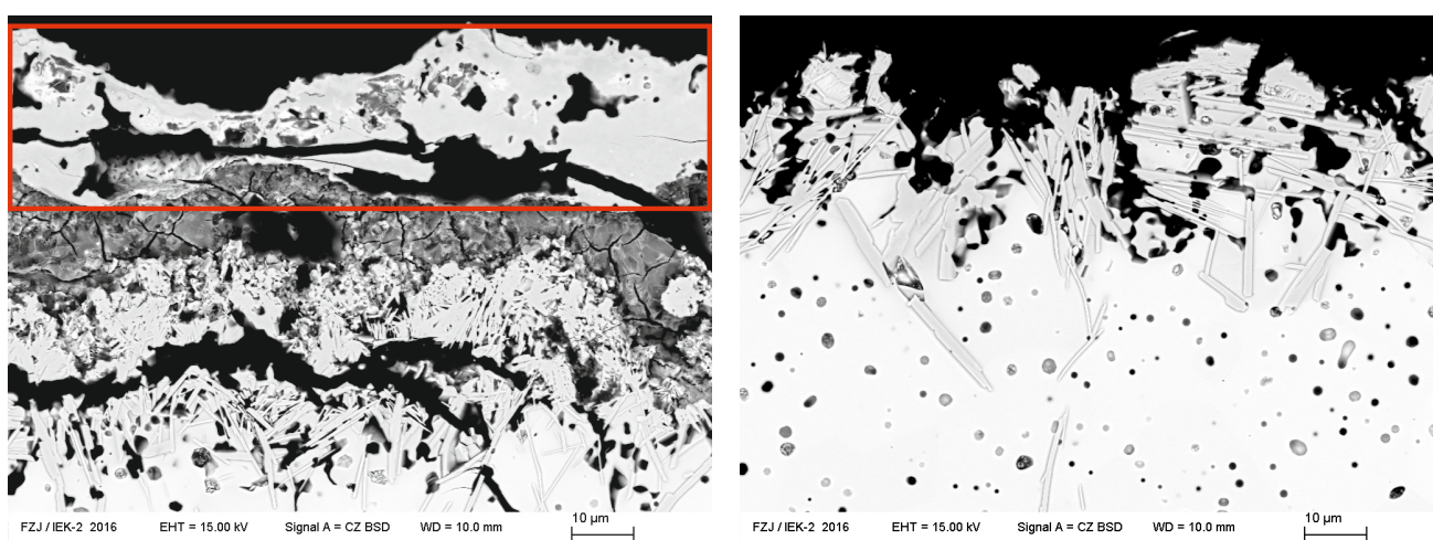
(a) Deposition of 10–20 μm dense silica layer at the membrane surface.
