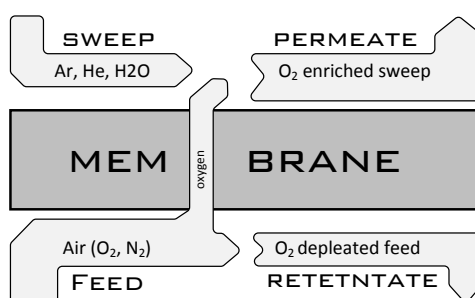
Figure 2. Simplified principle of oxygen permeation through a membrane in 4-end sweep gas mode.
