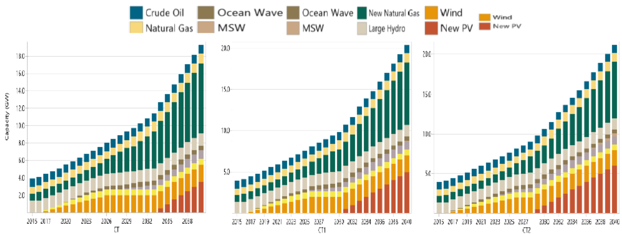
Figure 6. Installed capacity in CO 2 tax scenarios.
