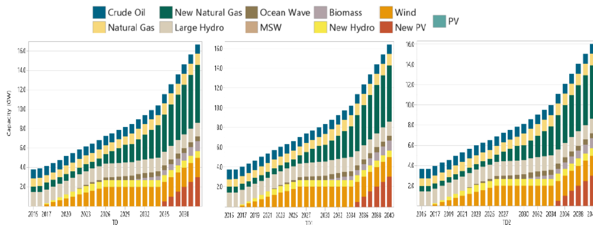
Figure 8. Installed capacity in transmission and distribution losses scenarios.
