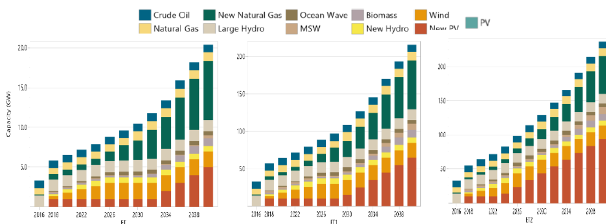
Figure 4. Installed capacity in CO 2 emission target scenarios.
