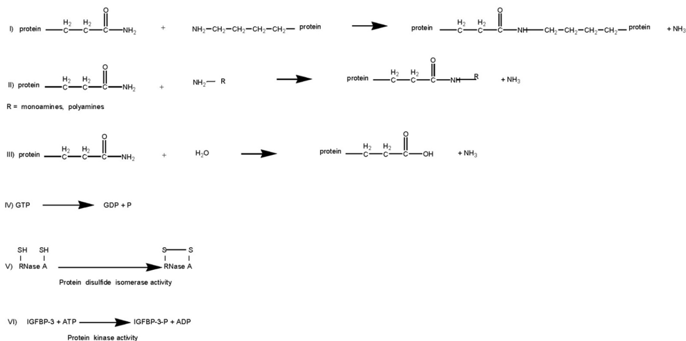
Figure 1A. Examples of reactions catalyzed by TG: (I) acyl transfer between the \gamma -carboxamide group of a protein/polypeptide glutamyl residue and the \epsilon -amino group of a protein/polypeptide lysyl residue; (II) attachment of a polyamine to the \gamma -carboxamide of a glutamyl residue; (III) deamidation of the \gamma -carboxamide group of a protein/polypeptide glutamyl residue; (IV) GTPase activity; (V) protein disulfide isomerase activity; (VI) protein kinase activity.
