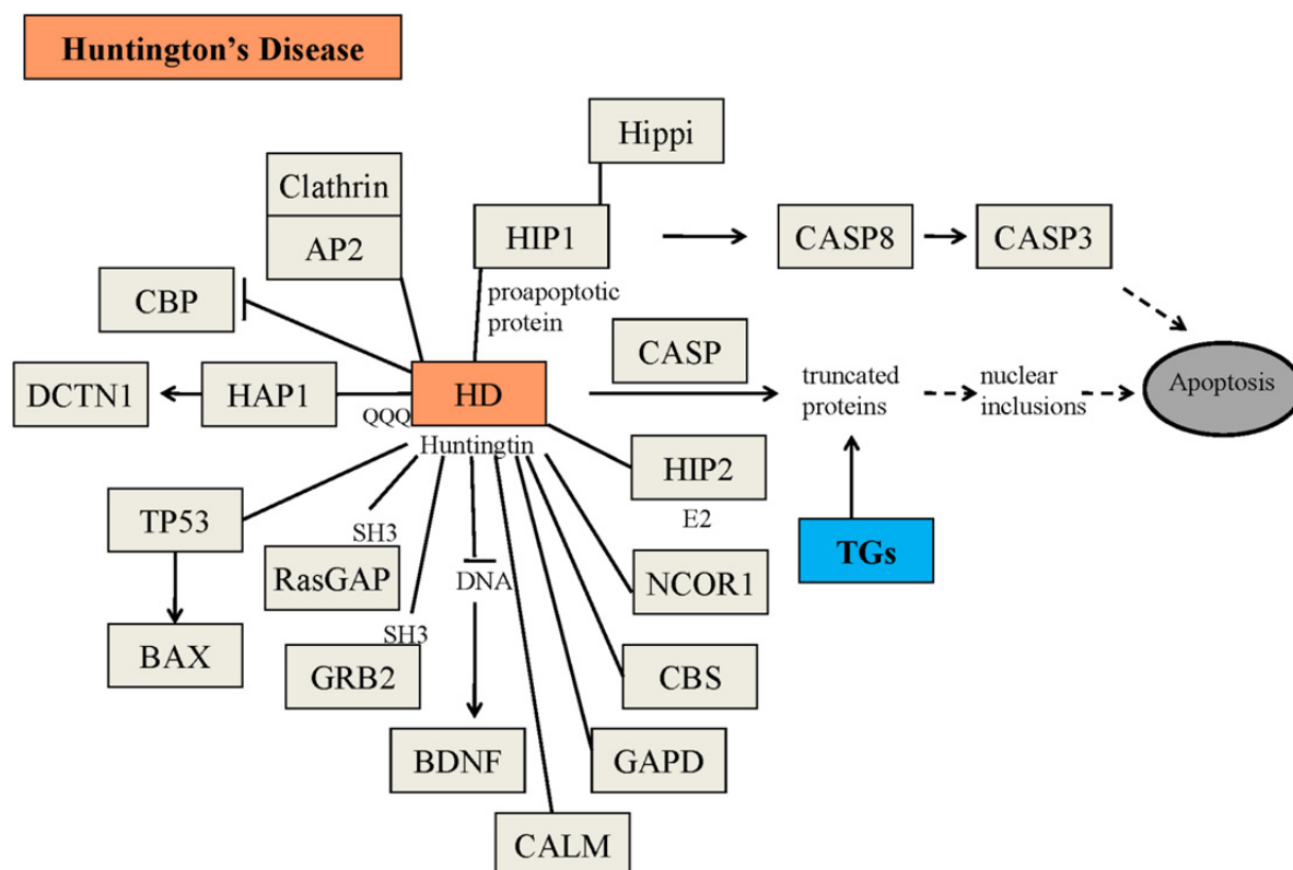
Figure 2. Possible physiopathological effects of the mutated huntingtin. Some of the physiopathological roles of mutated huntingtin, including the formation of nuclear inclusions, have been described in the Figure AP2 = adipocyte Protein 2; BAX = bcl-2-like protein 4; BDNF = brain-derived neurotrophic factor; CALM = calmodulin; CASP = caspases; CASP3 = caspase 3; CASP8 = caspase 8; CBP = CREB binding protein; CBS = cystathionine- \beta -synthase; DCTN1 = dynactin subunit 1; GAPD = glyceraldehyde-3-phosphate dehydrogenase; GRB2 = growth factor receptor-bound protein 2; HAP1 = huntingtin associated protein 1; HIP1 = huntingtin interacting protein 1; HIP2 = huntingtin interacting protein 2; Hippi =; HIP1 protein interactor; NCOR1 = nuclear receptor corepressor 1; RasGAP = p21Ras protein and GTPase-activating protein complex; TGs = transglutaminases; TP53 = tumor protein 53.
