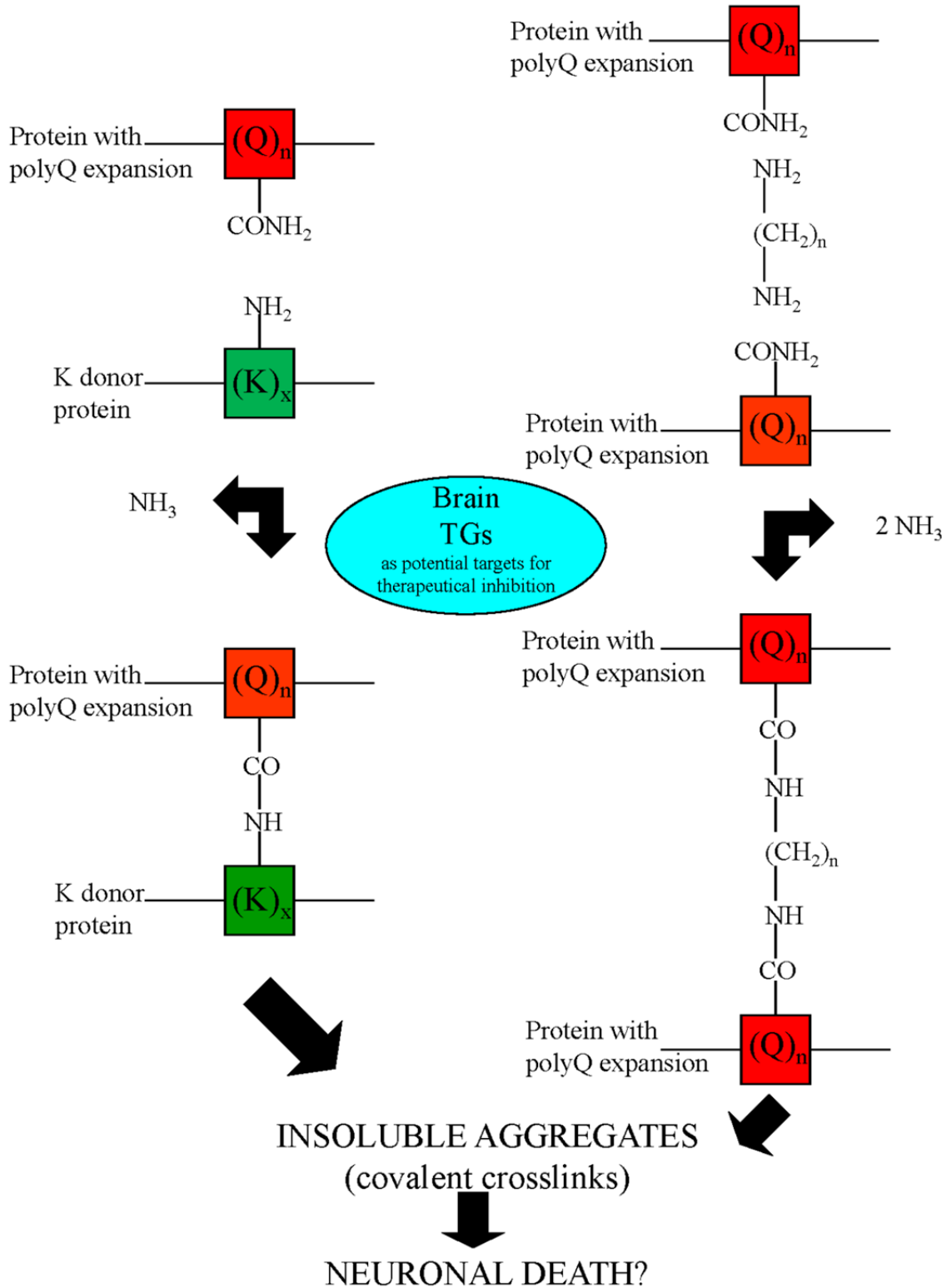
Figure 3. Possible mechanisms responsible for protein aggregate formation catalyzed by TGs. Transglutaminase activity could produce insoluble aggregates both by the formation of N^\epsilon -( \gamma -L-glutamyl)-L-lysine (GGEL) isopeptide bonds (left side of the figure) and by the formation of N,N-bis-( \gamma -L-glutamyl)polyamine bridges (right side of the figure) in the mutated huntingtin.
