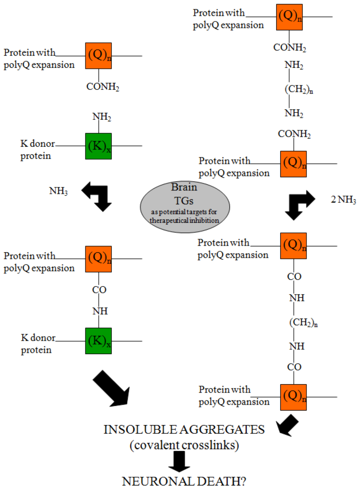
Figure 4. Possible mechanisms responsible for protein aggregate formation catalyzed by TGs. Transglutaminase activity could produce insoluble aggregates both by the formation of N^\epsilon -( \gamma -L-glutamyl)-L-lysine (GGEL) isopeptide bonds (left side of the figure) and by the formation of N,N -bis-( \gamma -L-glutamyl)polyamine bridges (right side of the figure) in the mutated huntingtin.
