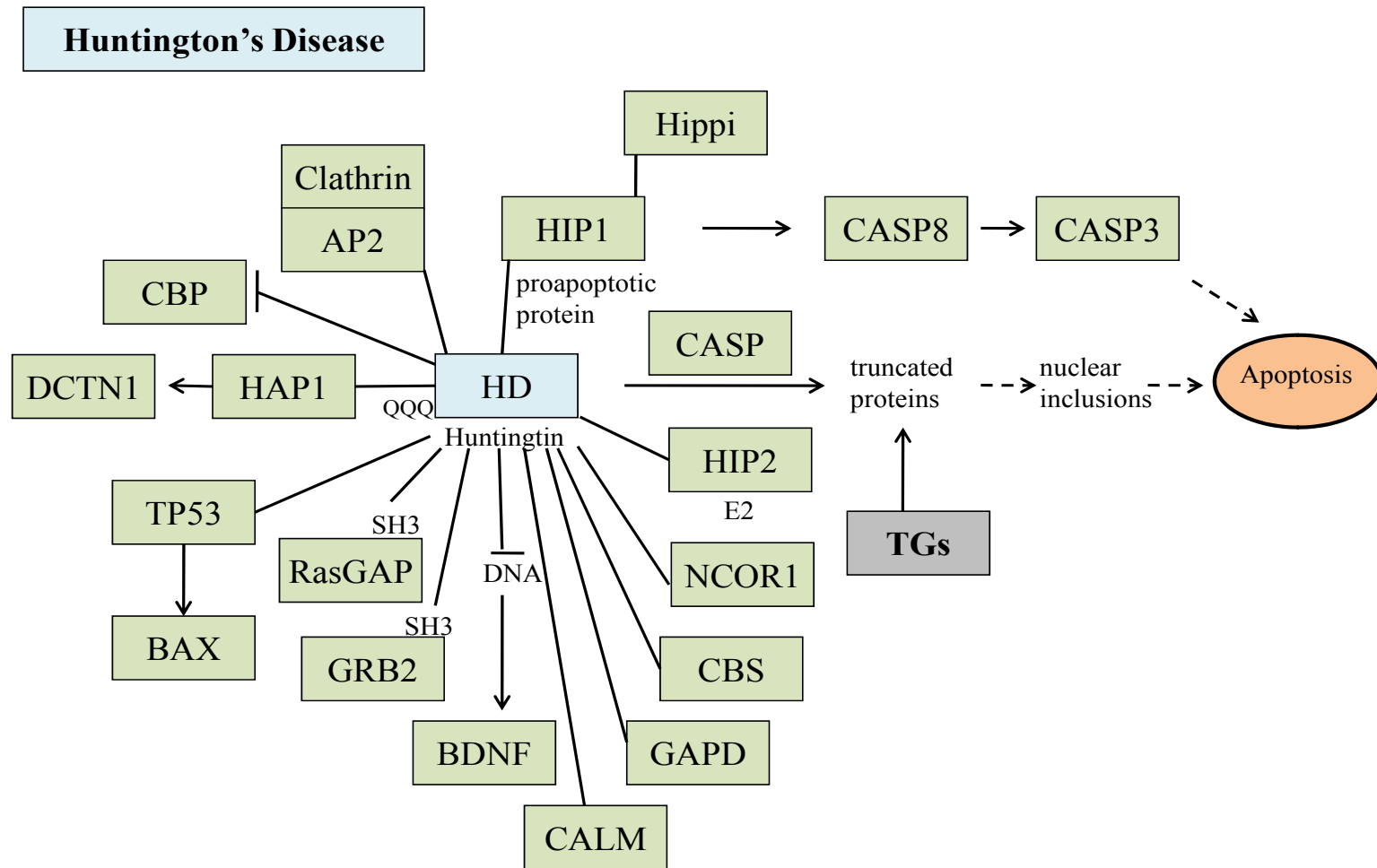
Figure 3. Possible physiopathological effects of the mutated huntingtin. Some of the physiopathological roles of mutated huntingtin, including the formation of nuclear inclusions, have been described in the figure.
